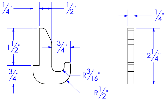
FP-HF12-LID LATCH LATCH, HYDRA FEEDER LID MATERIAL: 1/4" HRS
