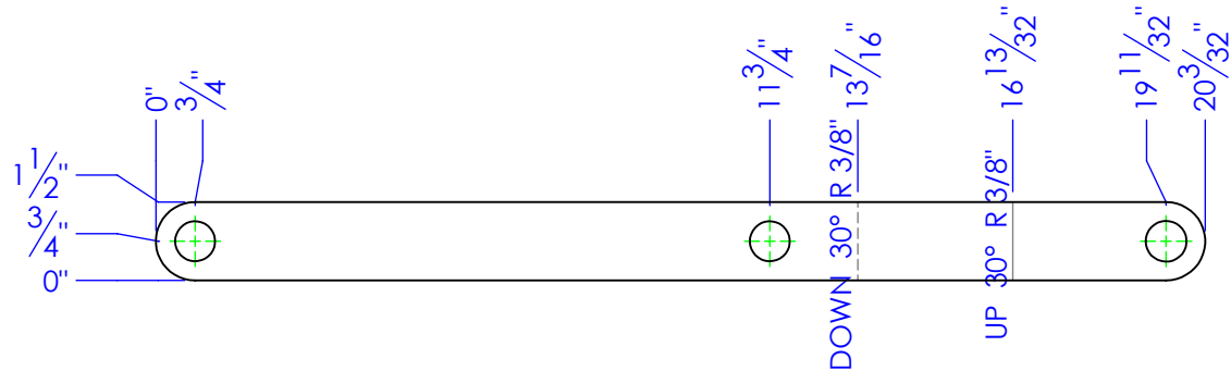
FP-HF12-LID LATCH LATCH, HYDRA FEEDER LID MATERIAL: 1/4" HRS
