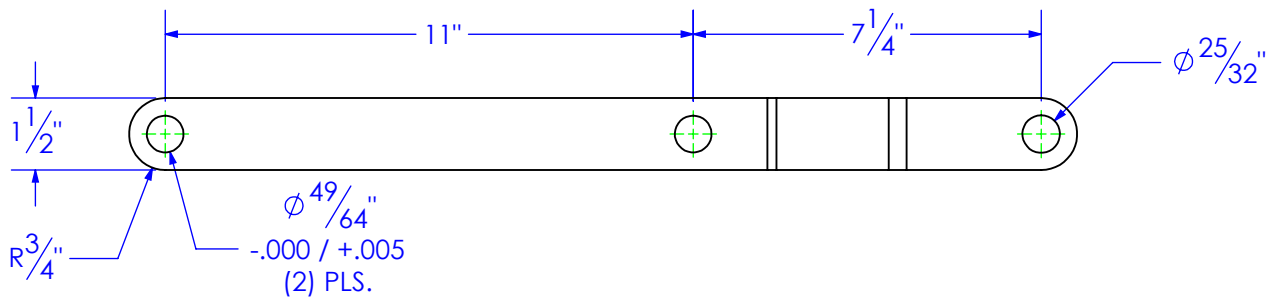
FP-HF12-HANDLE LEFT HINGE PIVOT HANDLE MATERIAL: 3/8" HRS
